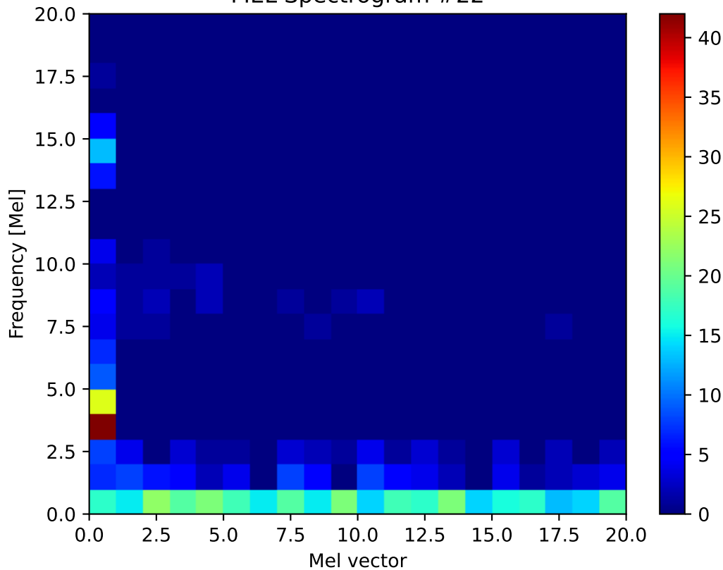
MEL Spectrogram #22
